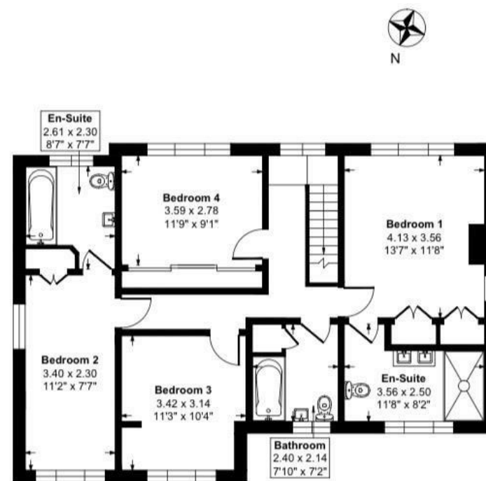
First Floor Approx. 84.6 sq. metres (910.9 sq. feet)
